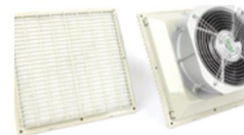
FKL6626 Enclosure Fan and Filter 320mm X 320mm 500/560m³/h
